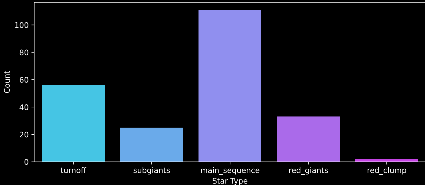
APOGEE DR17 Field: [080-45] Count plot of Star Type
