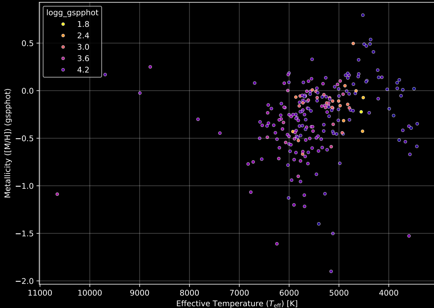
APOGEE DR17 Field: [080-45] Stellar Population Parameters (n= 227)
