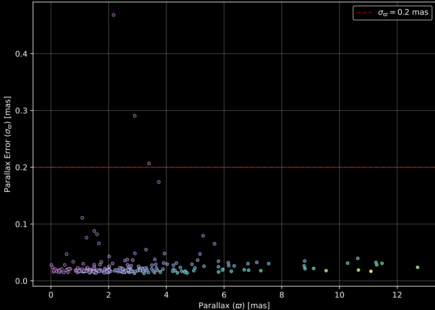
APOGEE DR17 Field: [080-45] Parallax Quality (n= 227)
