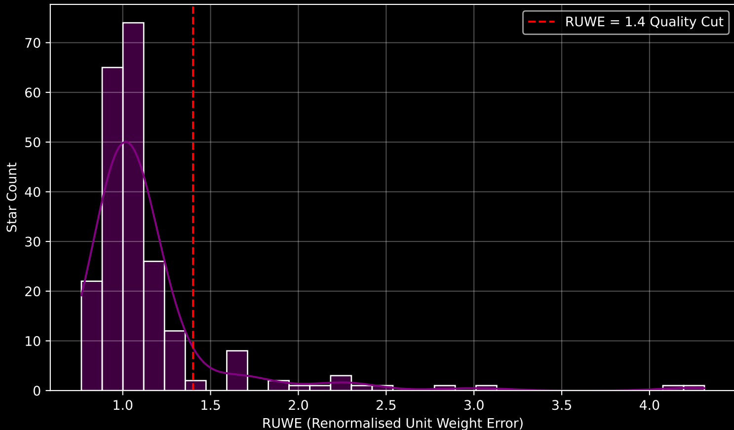
GAPOGEE DR17 Field [080-45] RUWE Distribution (n= 222)
