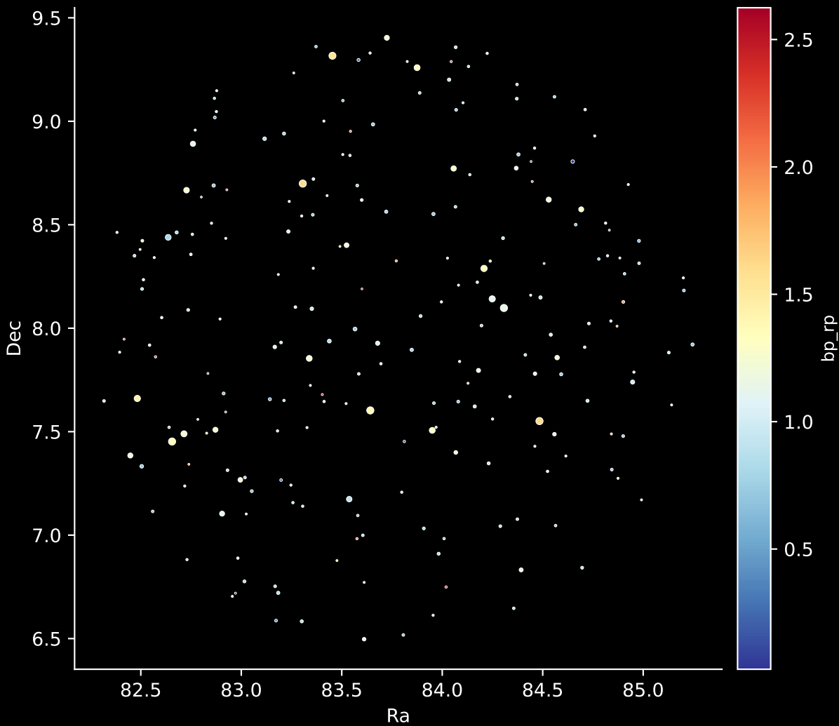
APOGEE DR17 Field: [080-45] Stars: 227
