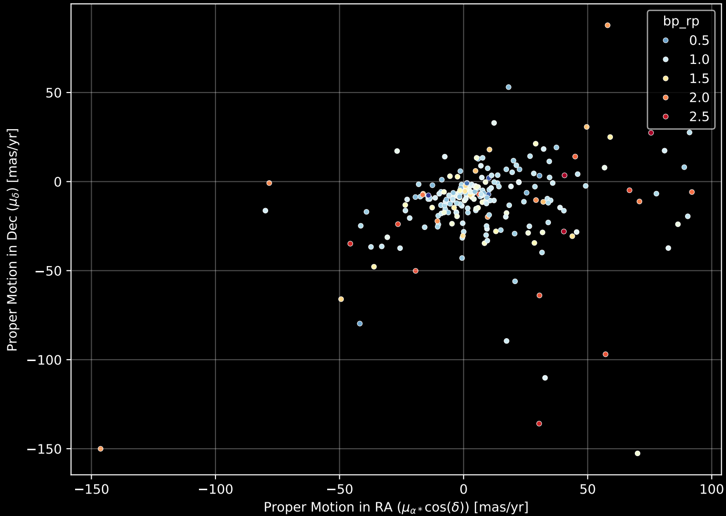
APOGEE DR17 Field: [080-45] Proper Motion Diagram (n= 227)
