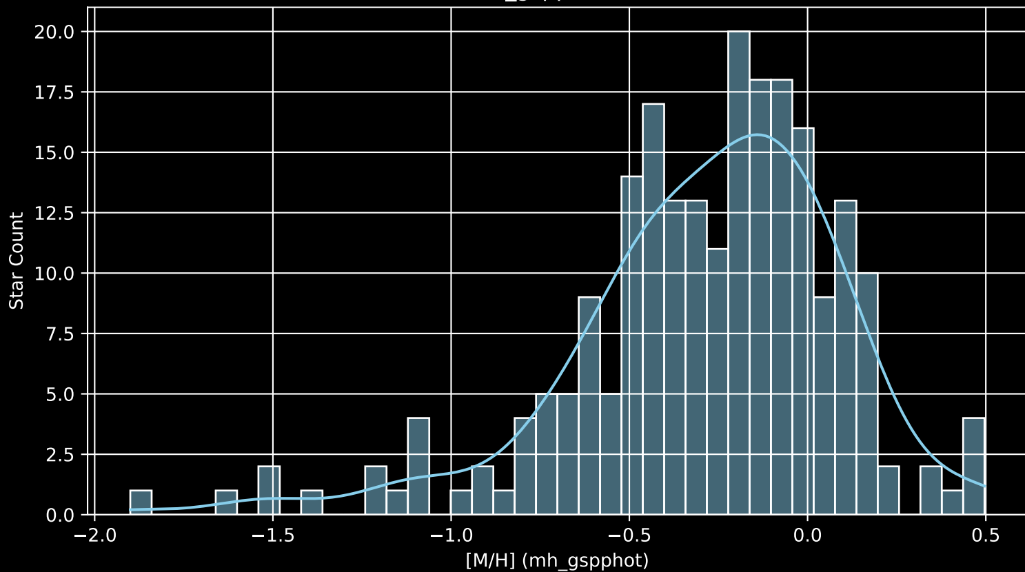
APOGEE DR17 Field: [080-45 [M/H] (mh_gspphot) (n= 225)
