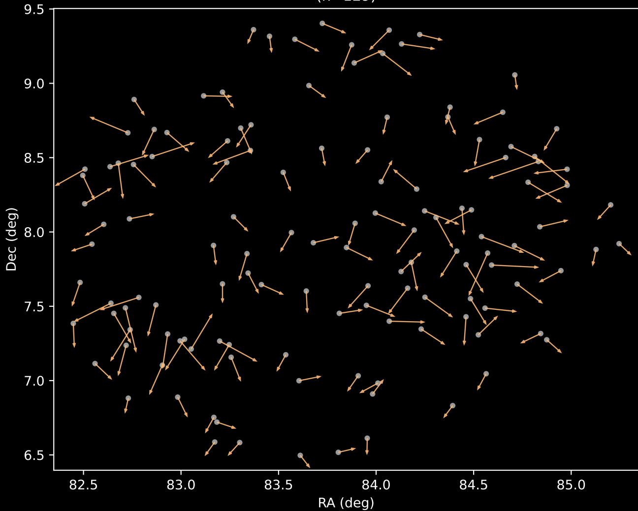
APOGEE DR17 Cluster 3 Proper Motion Vectors (n=129)
